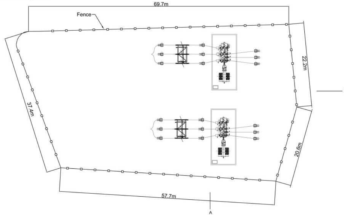
HV Transformer Compound
