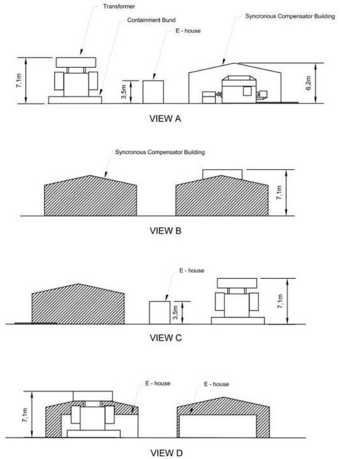
Indicative Elevation of Compound
