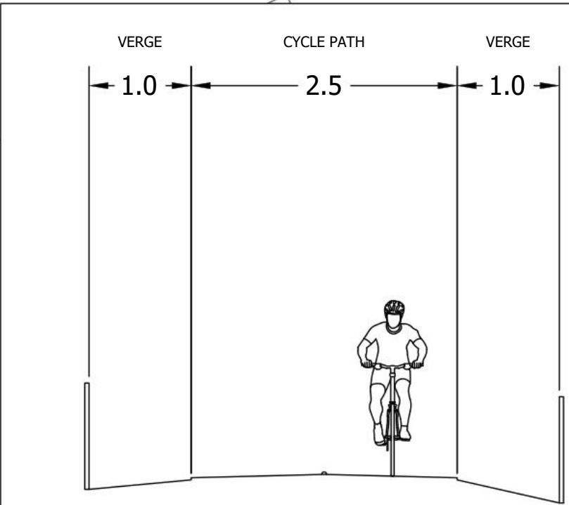
TYPICAL SECTION THROUGH FIELD SECTION C
