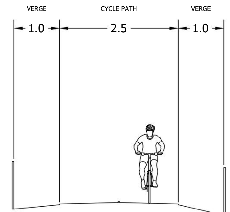
TYPICAL SECTION THROUGH FIELD SECTION C
