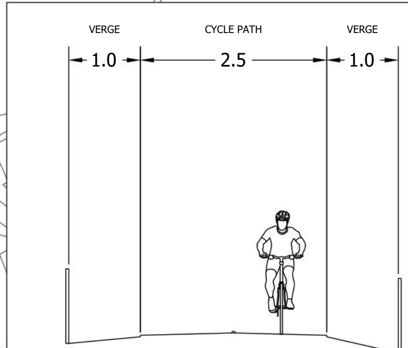
TYPICAL SECTION THROUGH FIELD SECTION C
