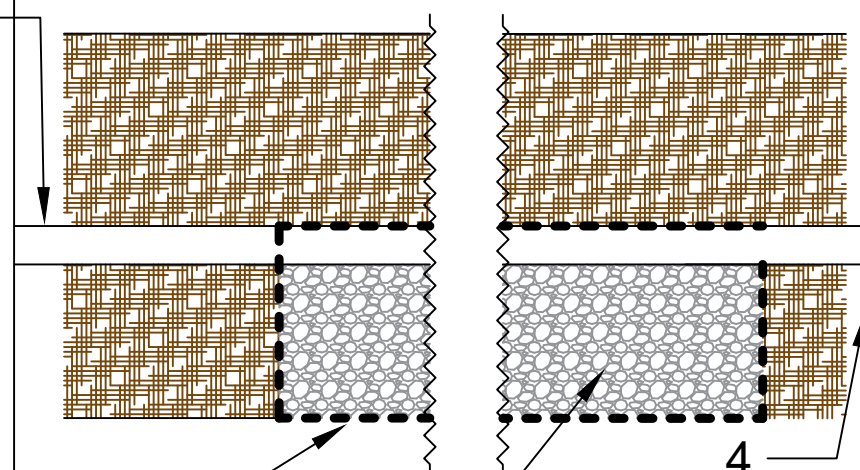
Partial Soakaway Design - Section BB (Not to Scale)
